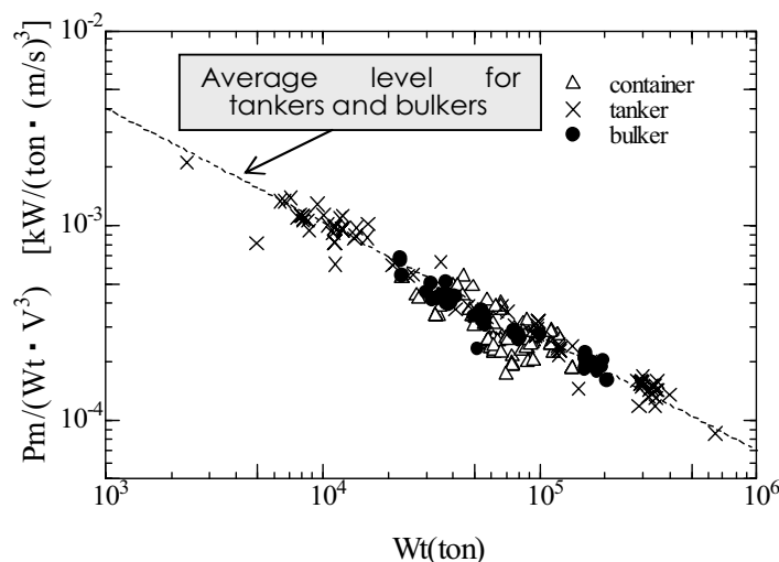
Fig.3 Resistance and propulsion performance of tanker, bulker and container ship
